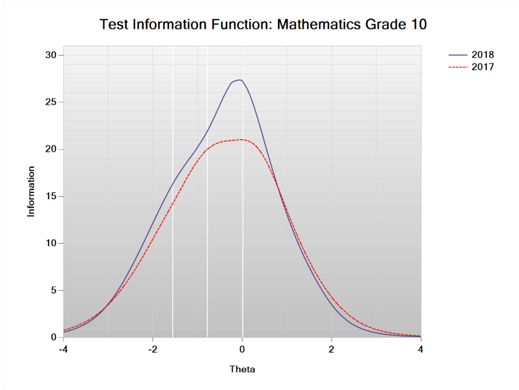
Figure I-4. 2018 Legacy MCAS: Test Information Function – Mathematics Grade 10
