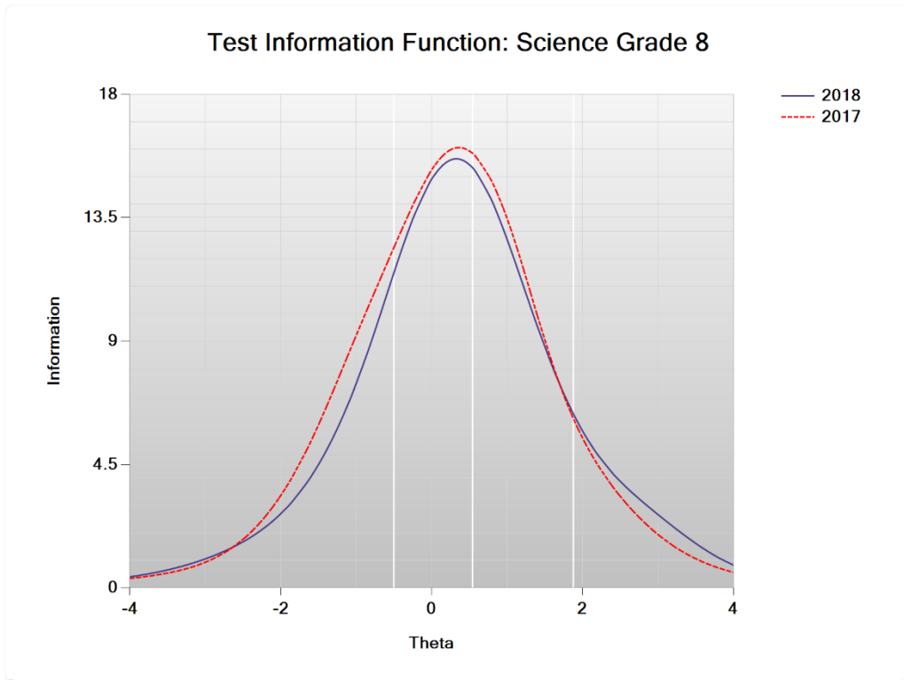
Figure I-16. 2018 Legacy MCAS: Test Information Function – Science Grade 8
